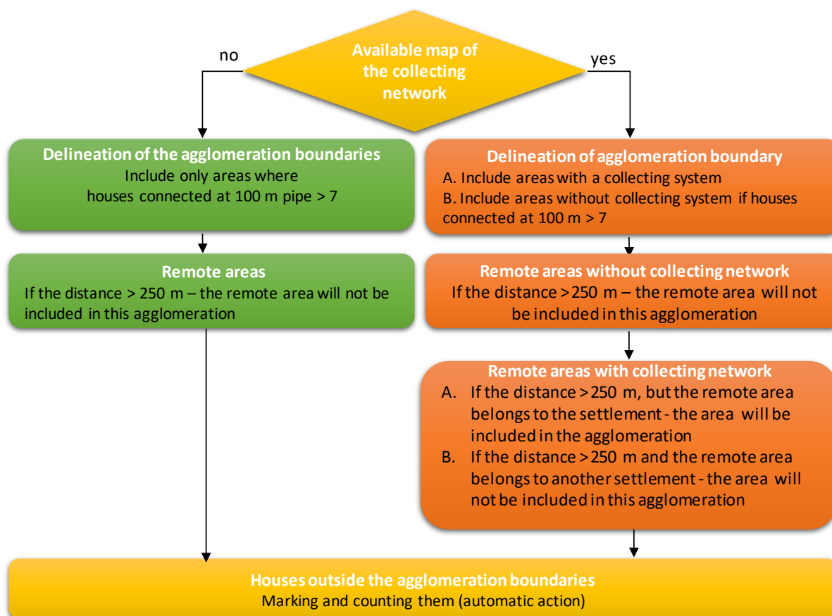
Figure 10: Algorithm for delineation of agglomeration boundaries
